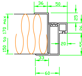
FRAME DETAIL 150- 170 PANEL
