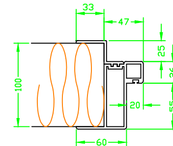
FRAME DETAIL 100mm PANEL
