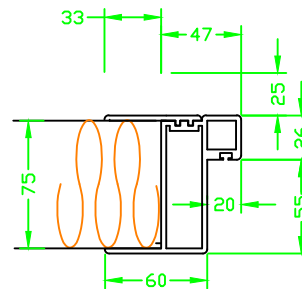
FRAME DETAIL 75mm PANEL
