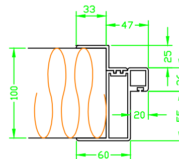
FRAME DETAIL 100mm PANEL
