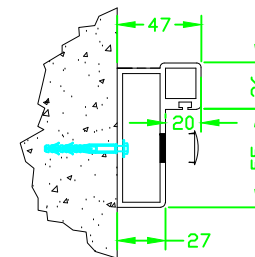
BRICKWORK OPENING
