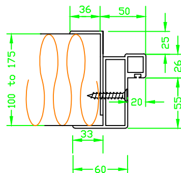
FRAME DETAIL 100- 175 PANEL
